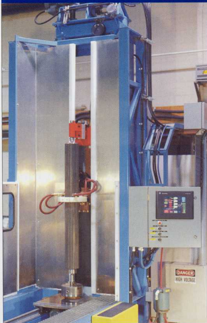
PRO MAC'S in house state of the art induction heat treating machine provides greater efficiency for on time delivery.
