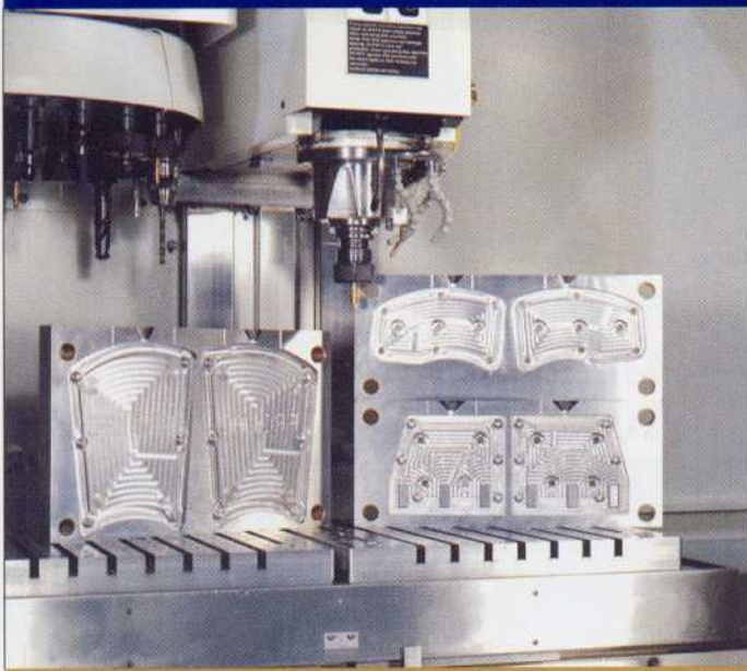
PRO MAC'S dedicated CNC Milling Machines create repeatable tolerances.
