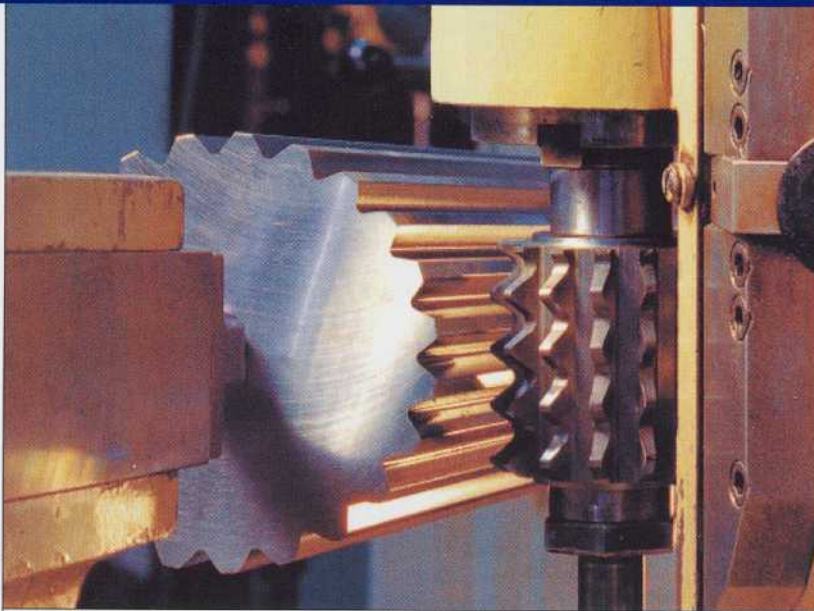
Hobbing Spline Shafts provides greater accuracy than index milling.
